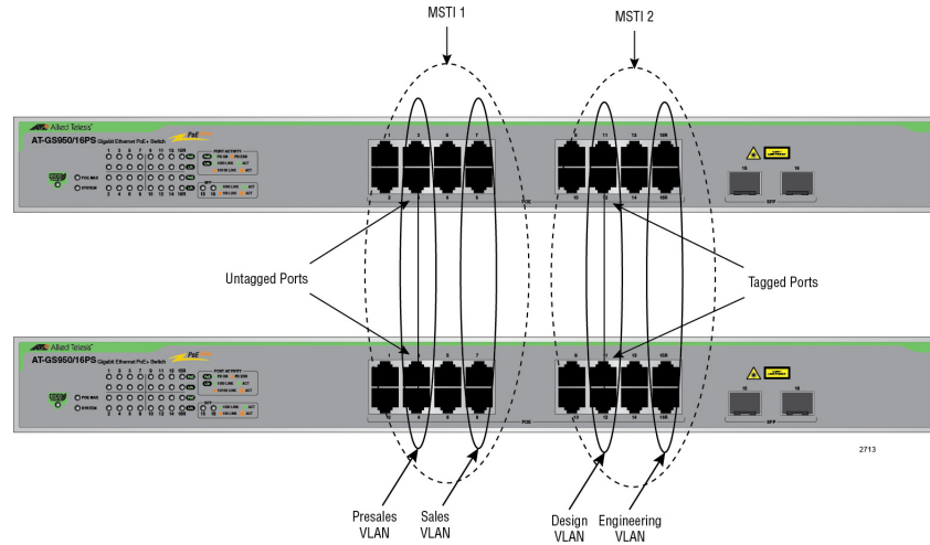
Figure 141. Multiple VLANs in a MSTI
